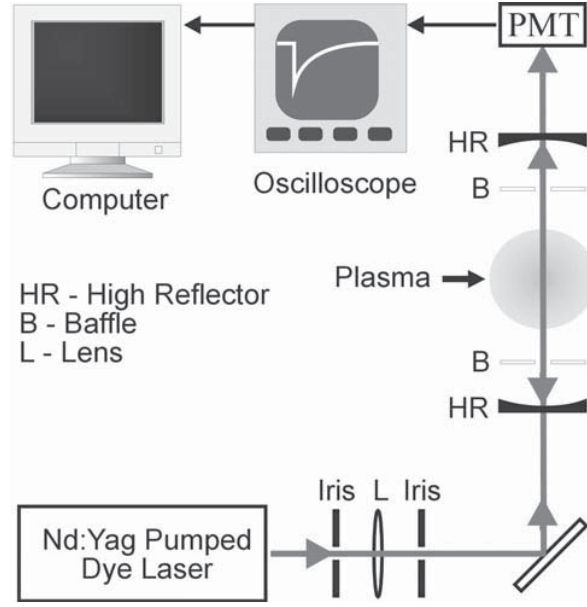
Figure 18. Schematic diagram of CRDS set-up used to probe N_2^+ .
