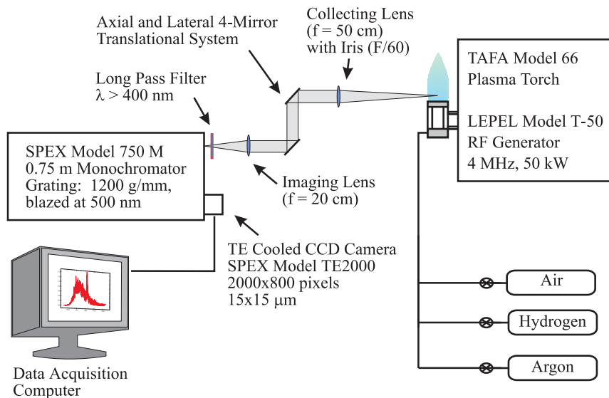
Figure 2. Typical experimental set-up for emission diagnostics.
