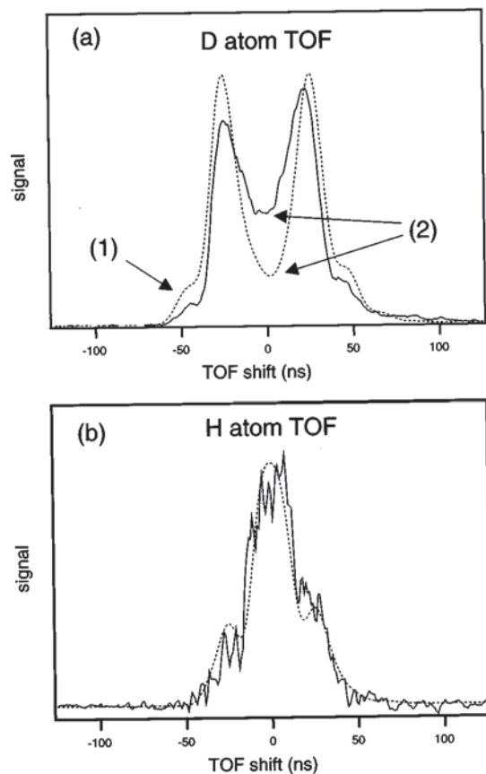
FIG. 16. (a) Experimental \text{D}^+ arrival profile (solid line) compared with a forward convoluted simulated profile (dashed line) using the QCT \text{HCl} DCSSs and vibrational branching ratio. The major deviations between the two profiles are marked and described in the text. (b) Same as (a) but for \text{H}^+ arrival profile.
