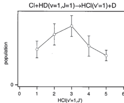
FIG. 2. \text{HCl}(v'=1) rotational state distribution for \text{Cl}+\text{HD}(v=1, J=1) at 0.065 eV mean collision energy. Data are obtained from REMPI spectra of the E(0,1) Q -branch, and populations are determined through the use of empirical correction factors. Error bars are statistical and represent one standard deviation.
