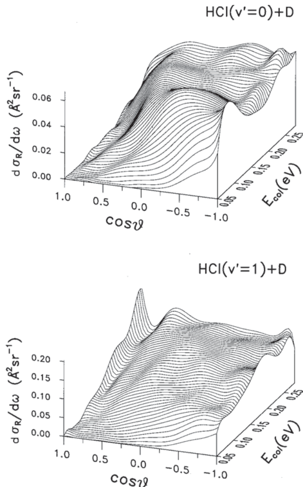
FIG. 8. 3D perspective of the collision energy dependent DCSs for the Cl+HD( v=1, J=1 ) reaction yielding HCl( v'=0 )+D (top) and HCl( v'=1 )+D (bottom) calculated quasiclassically on the G3 PES. Note the forward peak in the DCSs appearing at collision energies larger than 0.15 eV for the HCl( v'=1 )+D channel of the reaction.
