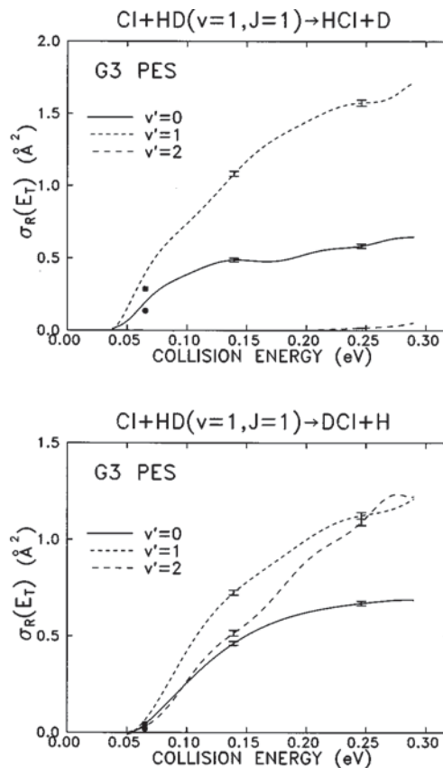
FIG. 7. Lines: QCT vibrationally state-resolved excitation functions for the Cl+HD( v=1, J=1 ) reaction. Solid symbols: QM reaction cross sections at the fixed collision energy E_{\text{col}}=0.065 eV.
