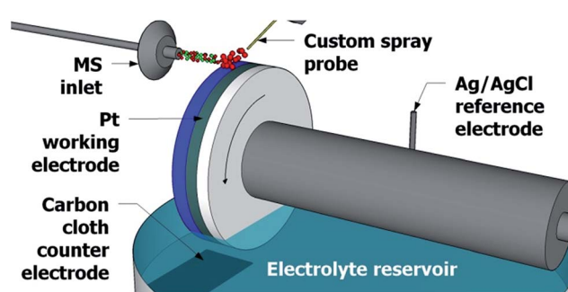
Fig. 1 The setup used for detection of electrochemical reaction intermediates, employing a rotating waterwheel electrode. Wheel rotation is indicated by the curved arrow.
