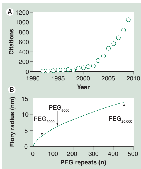
Figure 3. Polyethylene glycol background. (A) The number of literature citations for 'nanoparticle + PEG' as determined by Chemical Abstract Services indicates a progressive increase in the last decade. (B) The Flory radius of the PEG coil increases as a function of the number of monomers ( n ); see EQUATION 1. PEG: Polyethylene glycol.
