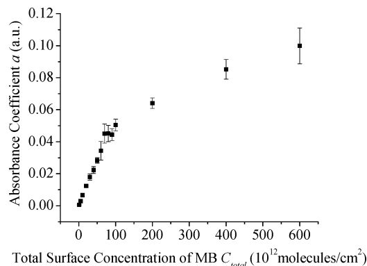
Figure 6. Absorption coefficient a versus the total surface concentration C_{total} .
