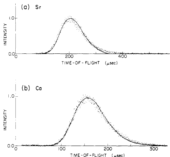
Figure 4. Typical time-of-flight spectra: (a) \text{Sr}(^3\text{P}) + \text{SF}_6 ; (b) \text{Ca}(^3\text{P}) + \text{SF}_6 . The solid curves are the best fit obtained with two adjustable parameters, v_0 and \sigma (see eq 3 and 4). Both (a) and (b) refer to the entries in Table II for the higher v' value.
