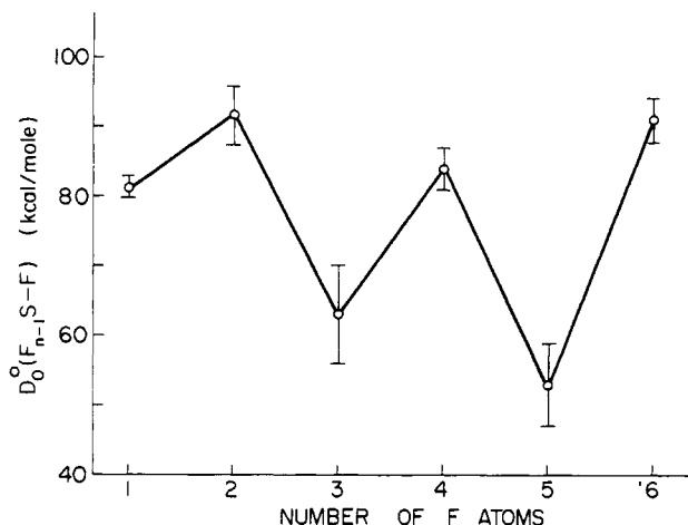
Figure 6. The sulfur fluoride bond dissociation energies as a function of the number of fluorine atoms.
