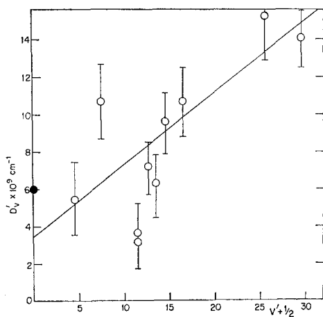
FIG. 2. Experimental values for D_v' . The filled point at v=0 is the Dunham predicted value, D_e=4B_e^3/\omega_e^2 .
